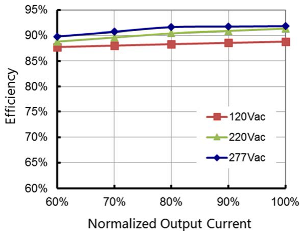
Efficiency vs. Load (24V Model)
