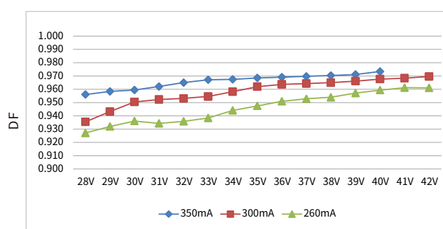
Displacement factor vs. voltage
