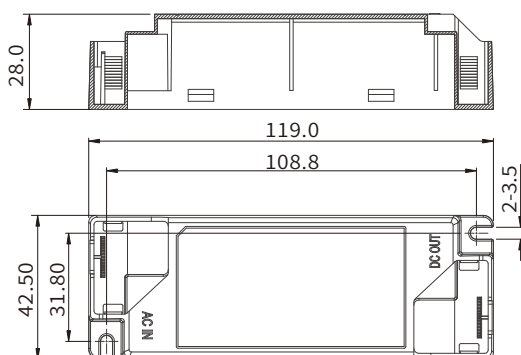
BK-PQL060
