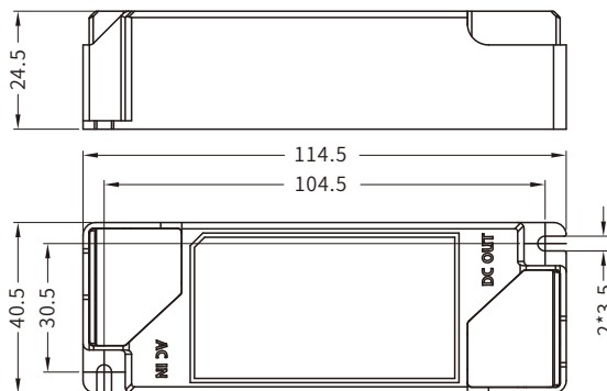
BK-PQL018/BK-PQL022
