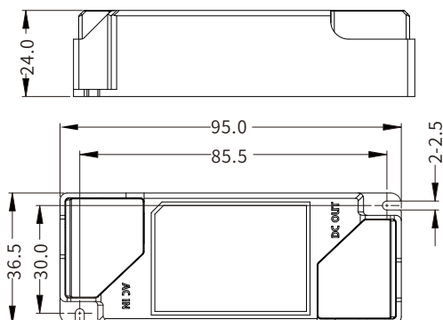
BK-PQL009/BK-PQL013
