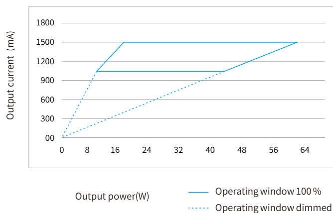
Operating window
