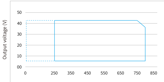
Operating window
