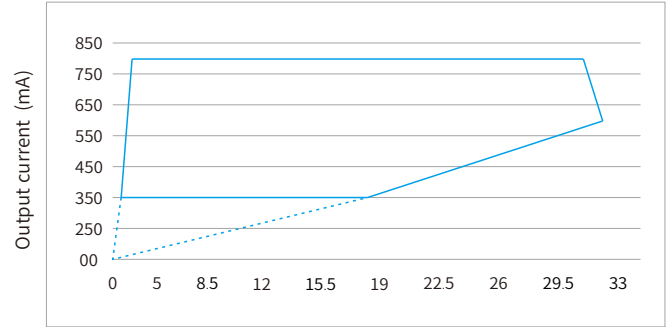
Operating window
