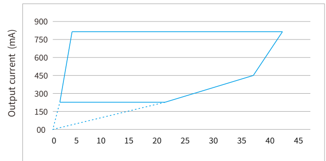
Operating window
